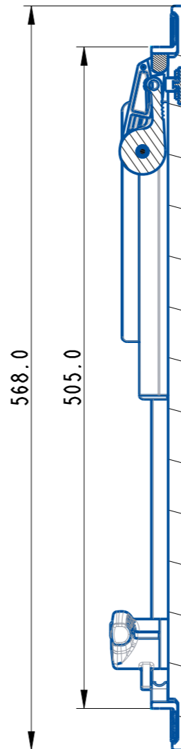
SECTION X-X
