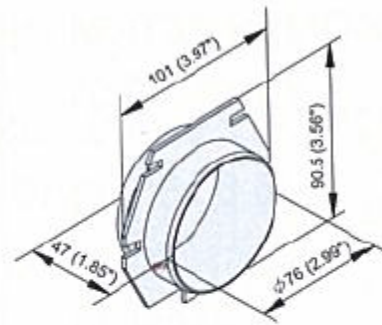
504-0237001 MOUNTING CLAMP & COLLAR SET
